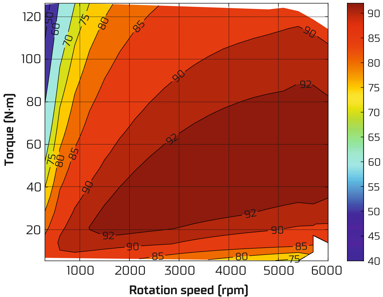
Efficiency map motor [%]
